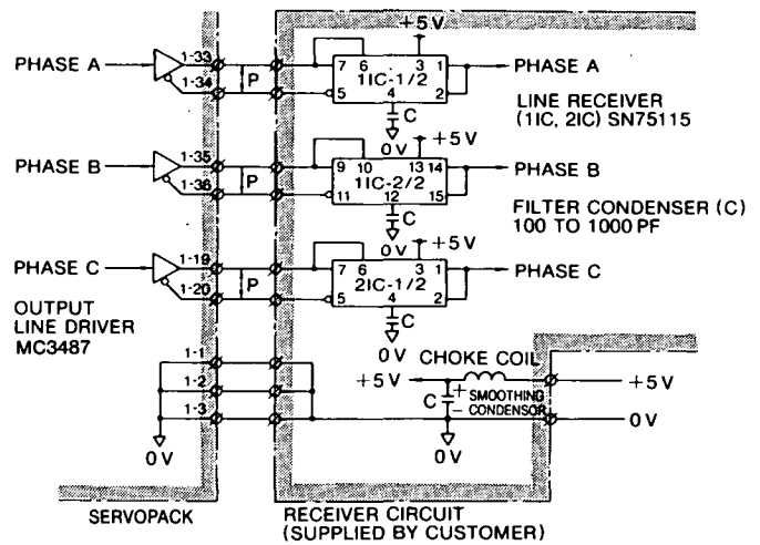
Fig. 6.8 Output Circuit and Receiver Circuit
