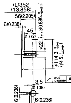
• Type USASEM-30AC2K* Type USASEM-30AC2KB†
