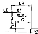
Detail of Shaft Extension
