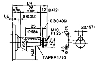
Detail of Shaft Extension
