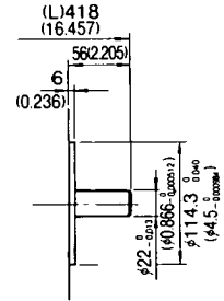
• With brake Type USASEM-30AC20B
