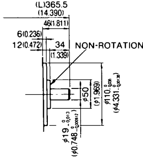
• With brake Type USASEM-15AC20B
