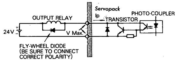
Fig. 6.7 Output Circuit
