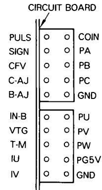
Fig. 6.18 Check Terminal Arrangement
