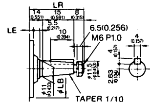
Detail of Shaft Extension
