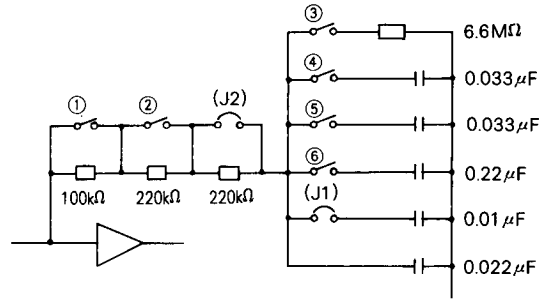
Fig. 6.15 Speed Amplifier PI Constant (SW3-① to ⑥)
