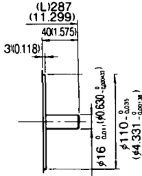
• With brake Type USASEM-08AC20B
